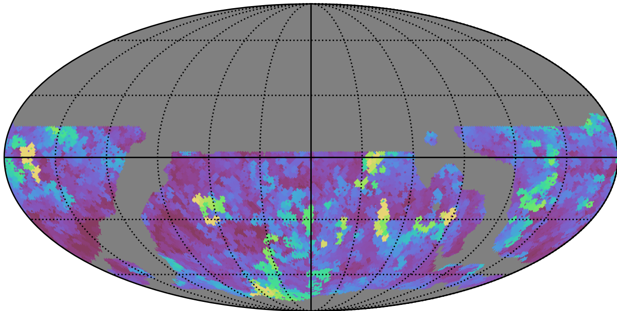
weather_cloudso10v3.4_10yrs WFD z band: Max seeingEff
