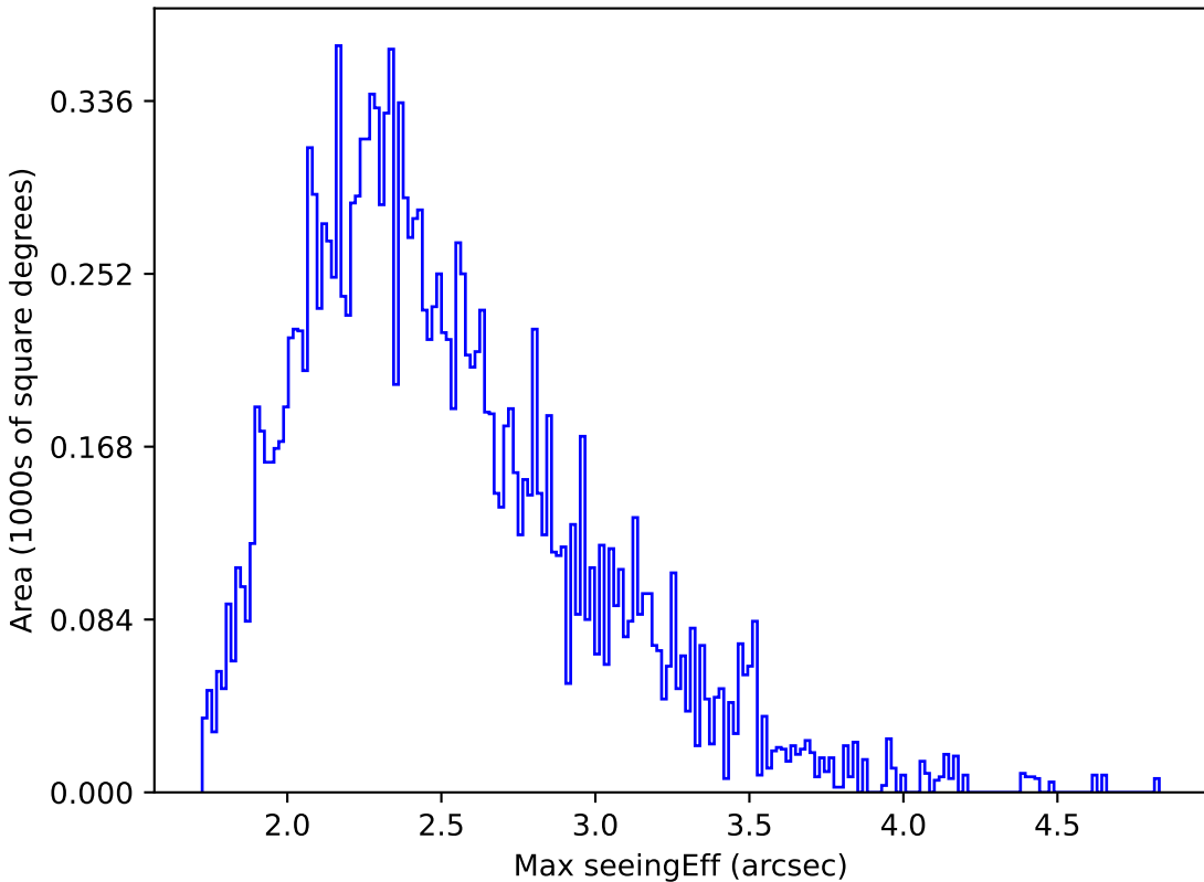
weather_cloudso10v3.4_10yrs WFD y band: Max seeingEff
