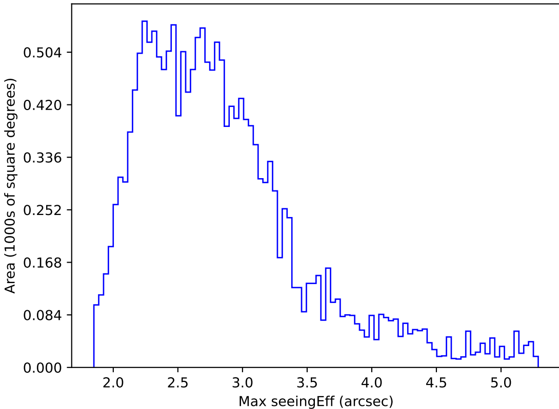
weather_cloudso10v3.4_10yrs WFD i band: Max seeingEff
