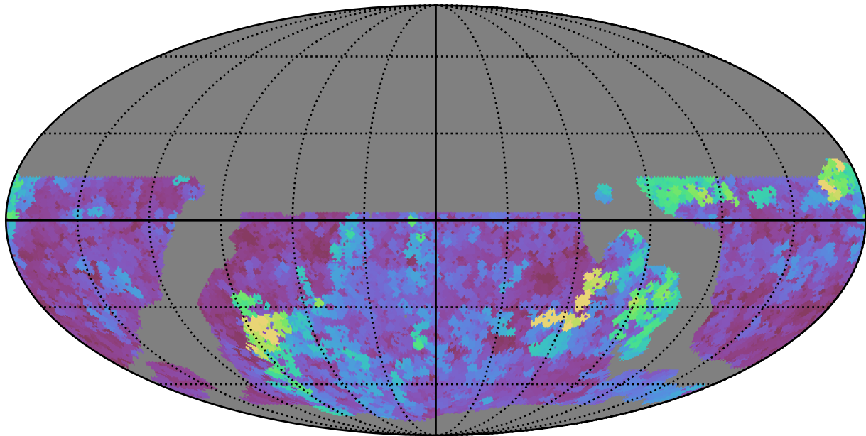
weather_cloudso10v3.4_10yrs WFD g band: Max seeingEff
