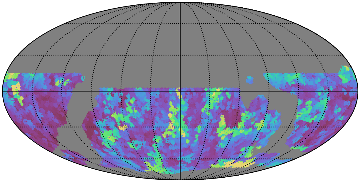
weather_cloudso10v3.4_10yrs WFD all bands: Max seeingEff
