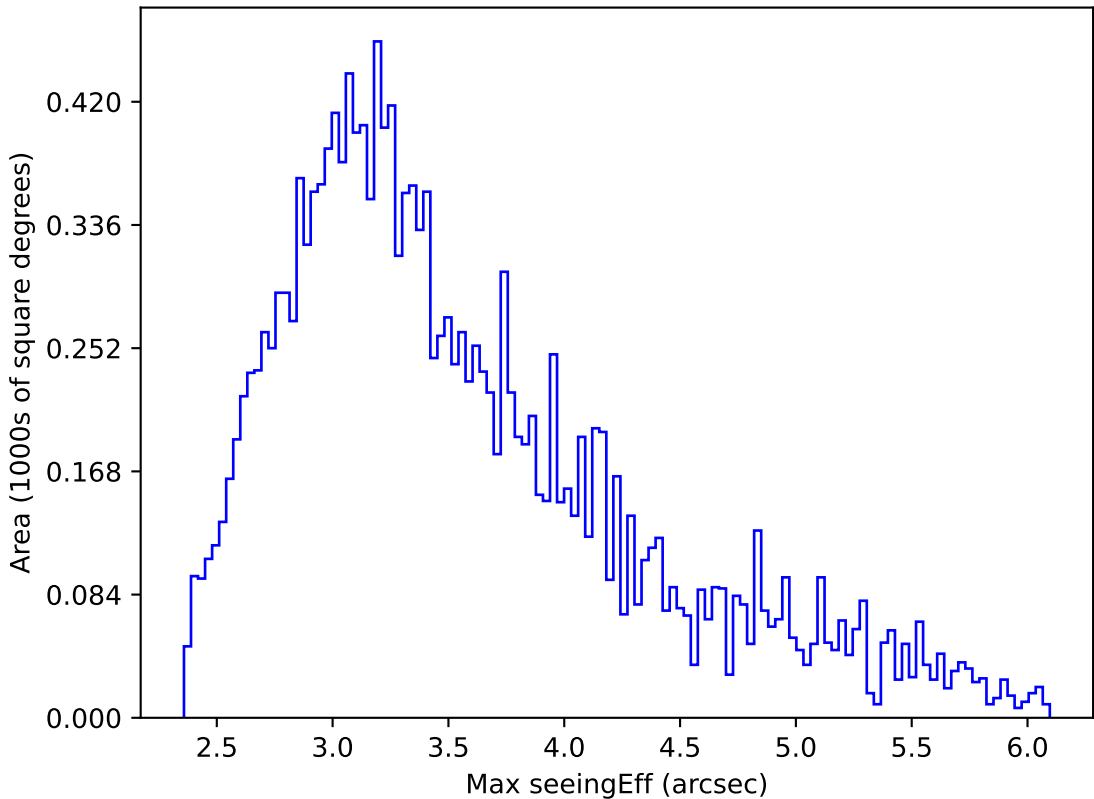
weather_cloudso10v3.4_10yrs WFD all bands: Max seeingEff
