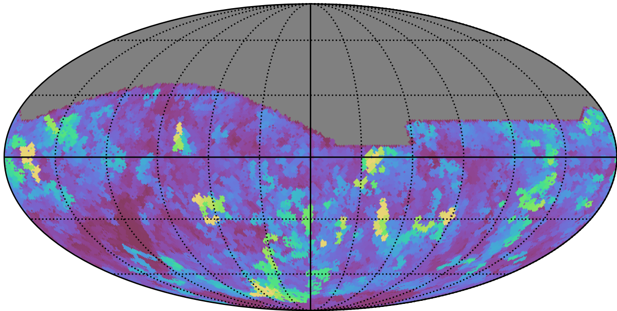
weather_cloudso10v3.4_10yrs All sky z band: Max seeingEff
