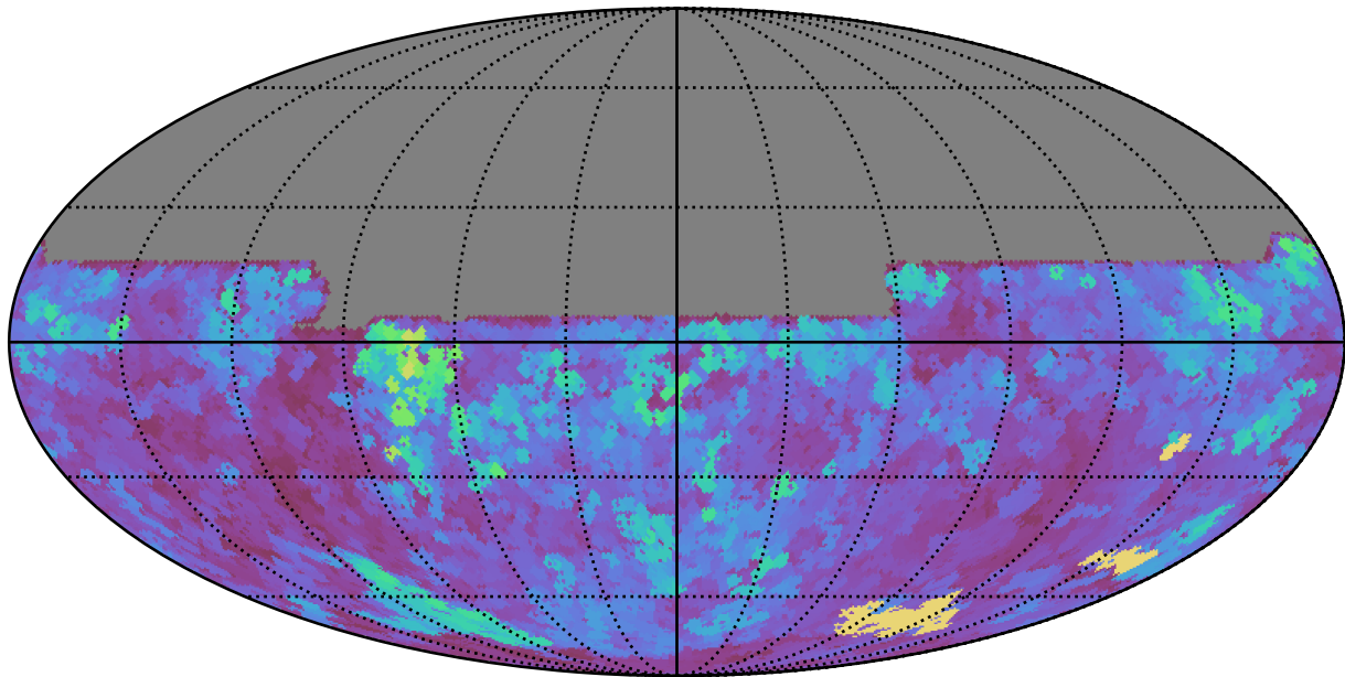
weather_cloudso10v3.4_10yrs All sky y band: Max seeingEff
