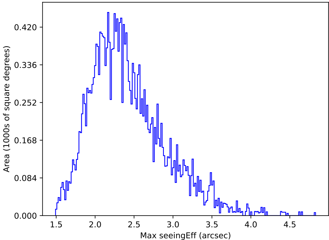
weather_cloudso10v3.4_10yrs All sky y band: Max seeingEff
