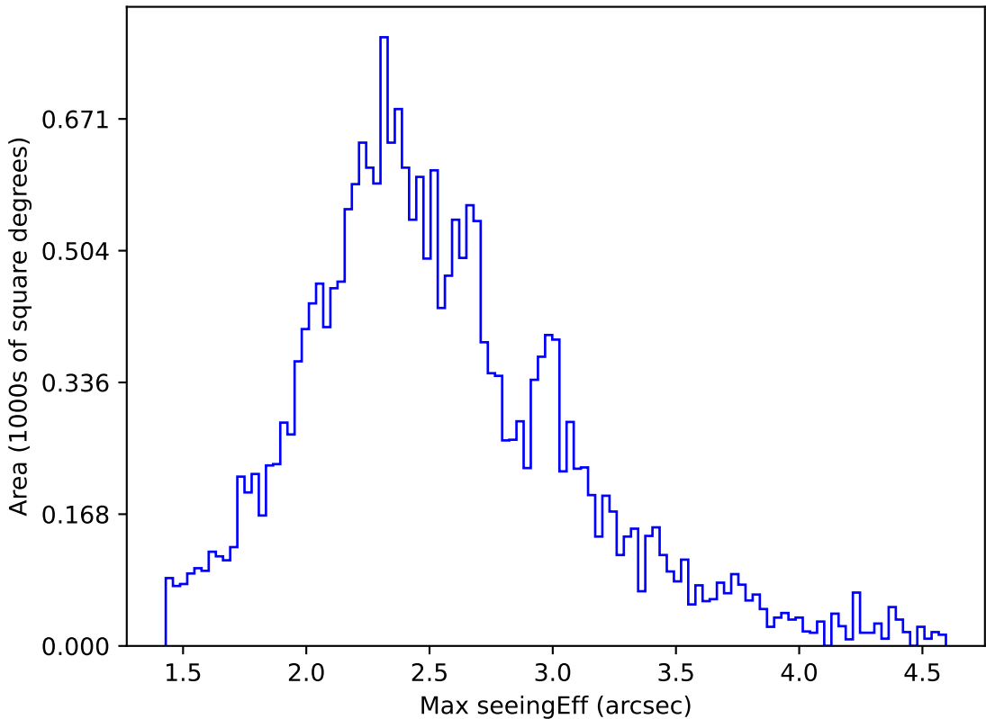
weather_cloudso10v3.4_10yrs All sky u band: Max seeingEff
