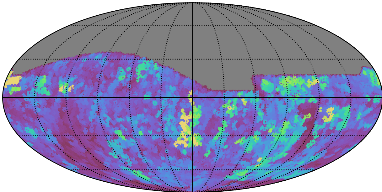
weather_cloudso10v3.4_10yrs All sky r band: Max seeingEff
