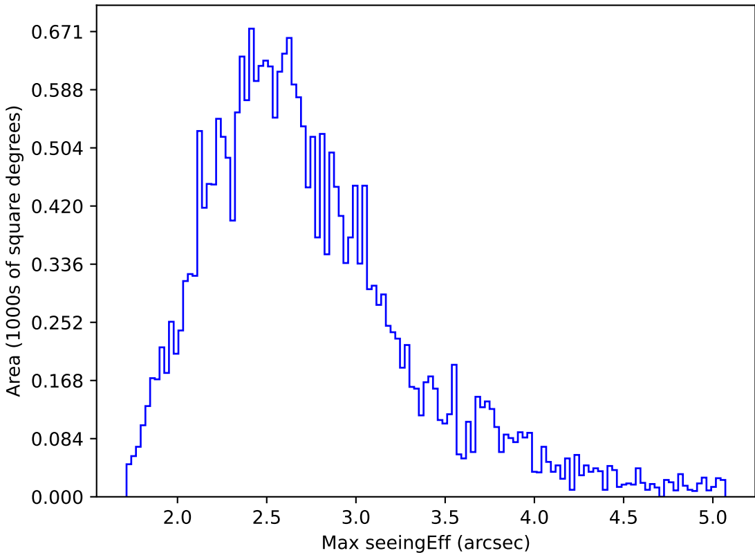
weather_cloudso10v3.4_10yrs All sky r band: Max seeingEff
