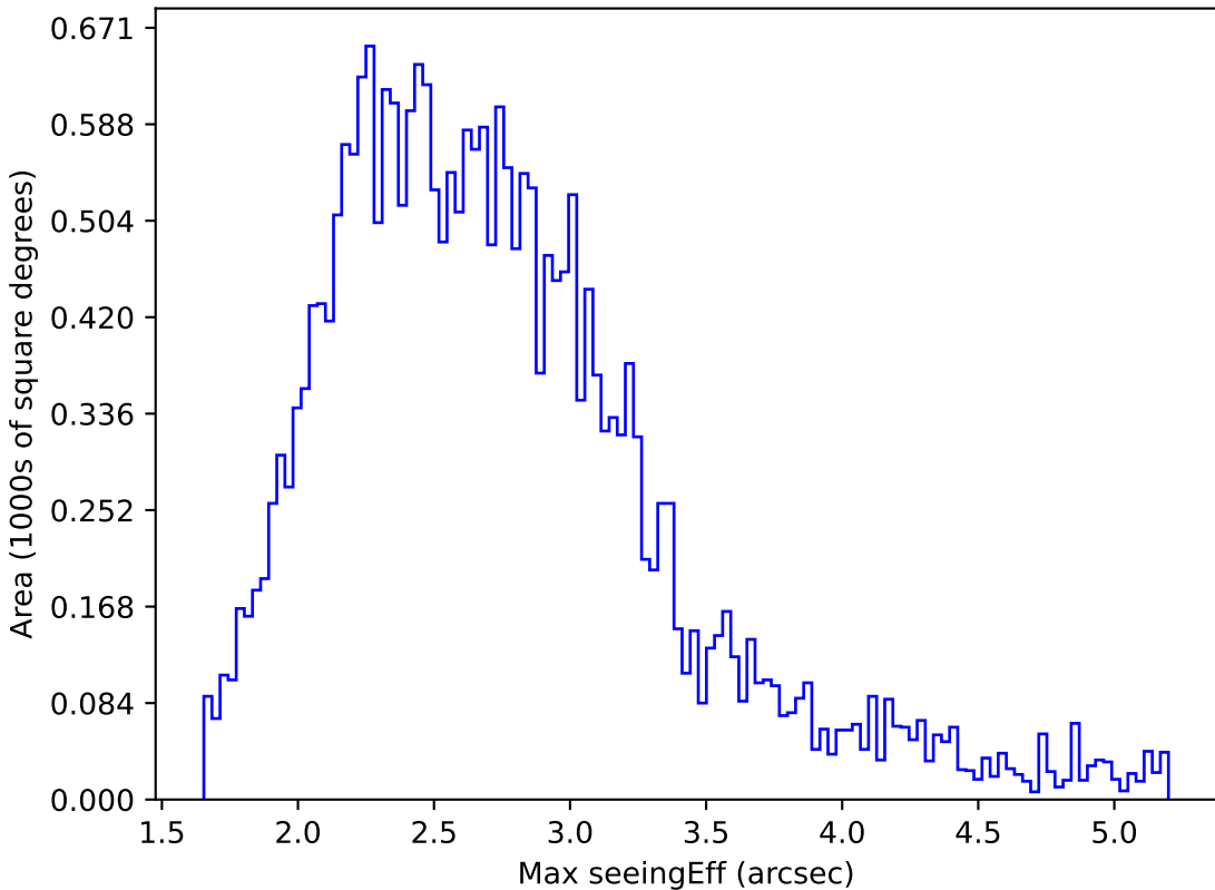
weather_cloudso10v3.4_10yrs All sky i band: Max seeingEff
