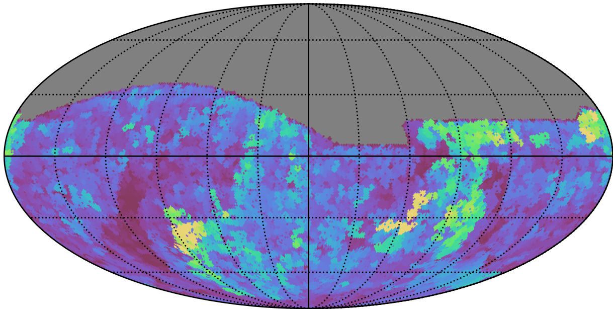
weather_cloudso10v3.4_10yrs All sky g band: Max seeingEff
