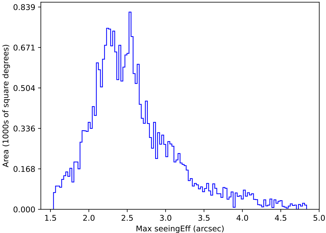
weather_cloudso10v3.4_10yrs All sky g band: Max seeingEff
