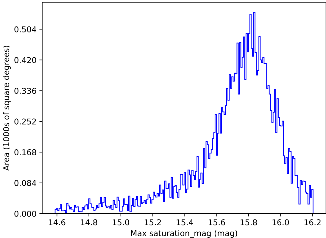
weather_cloudso10v3.4_10yrs All sky all bands: Max saturation_mag
