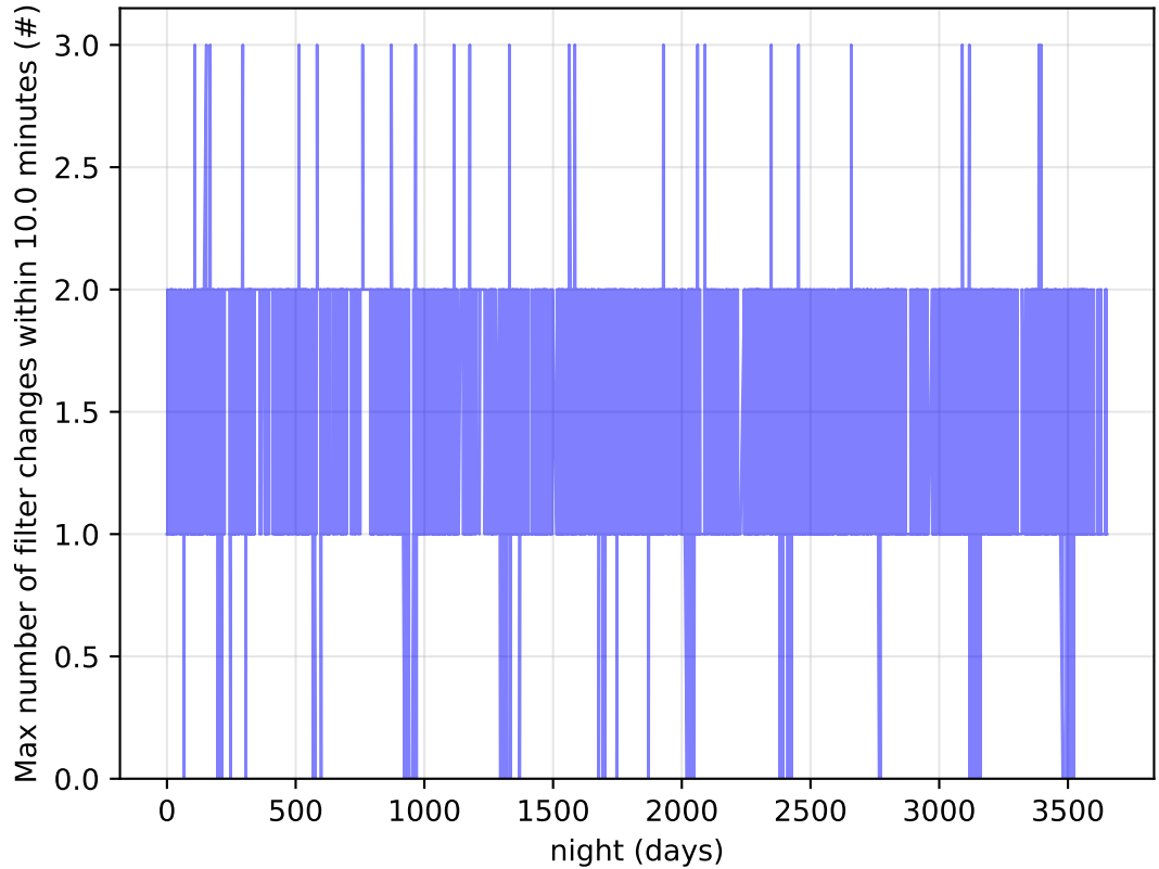
weather_cloudso10v3.4_10yrs Per Night: Max number of filter changes within 10.0 minutes
