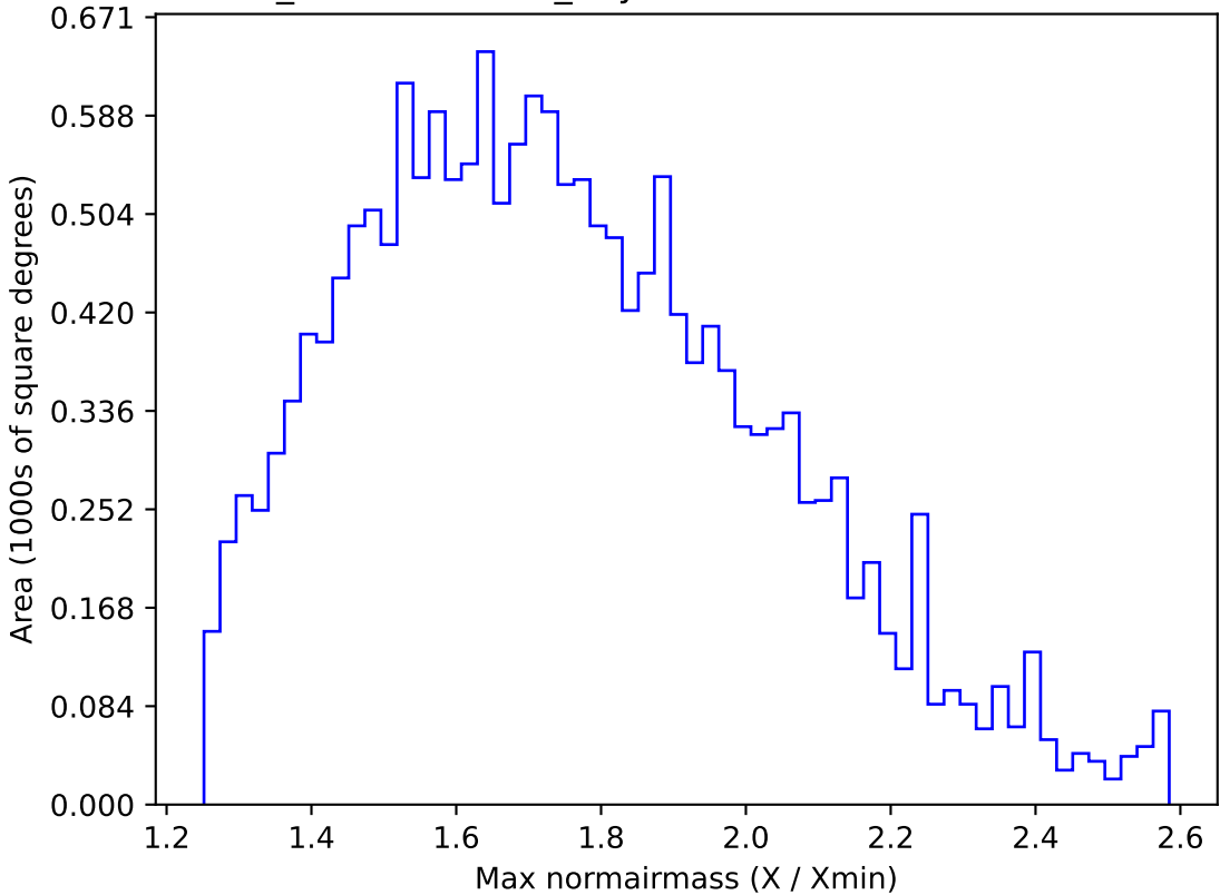
weather_cloudso10v3.4_10yrs WFD u band: Max normairmass
