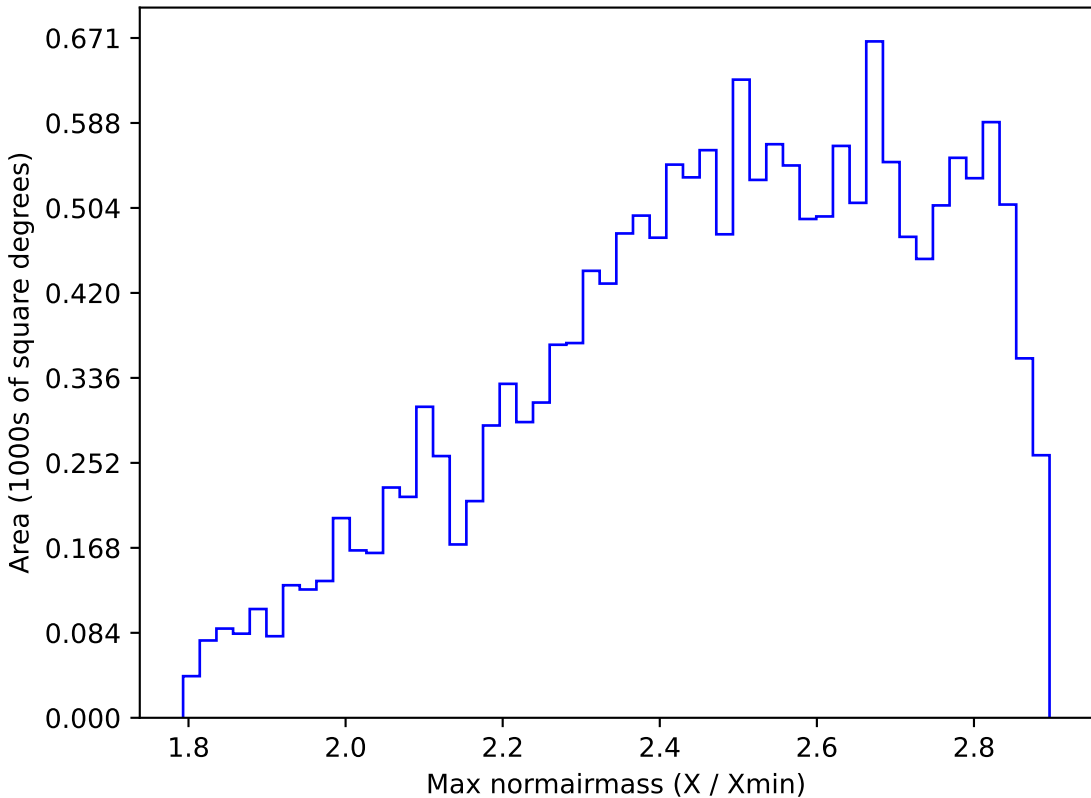
weather_cloudso10v3.4_10yrs WFD all bands: Max normairmass
