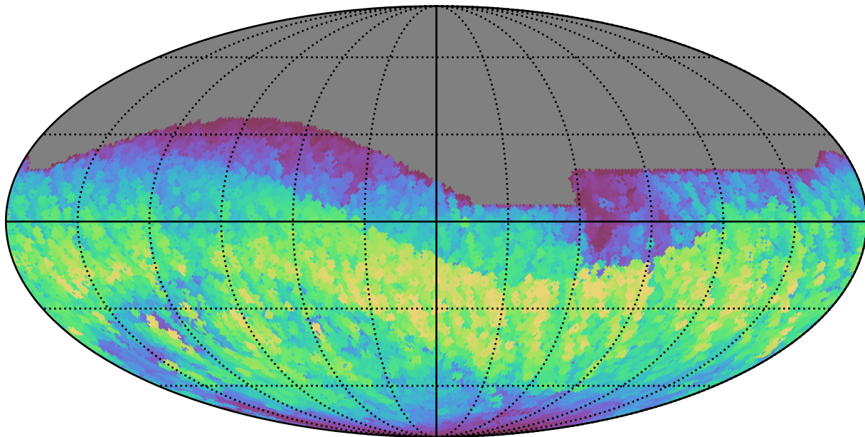
weather_cloudso10v3.4_10yrs All sky z band: Max normairmass
