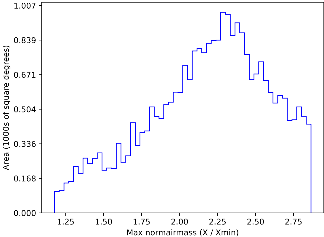
weather_cloudso10v3.4_10yrs All sky z band: Max normairmass
