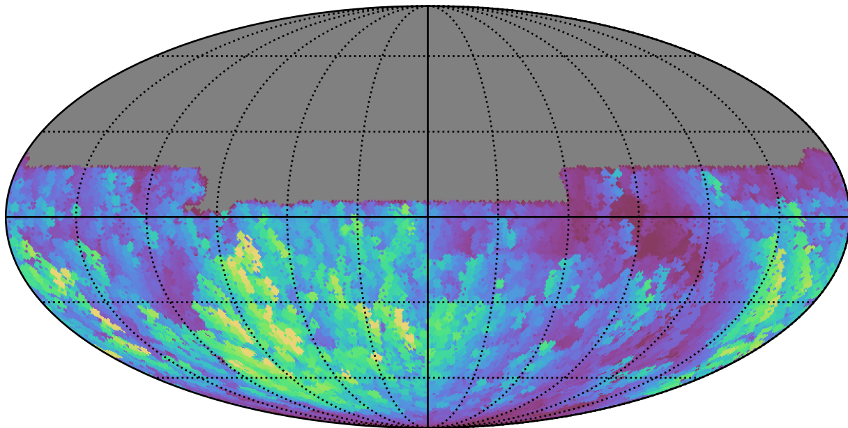
weather_cloudso10v3.4_10yrs All sky u band: Max normairmass
