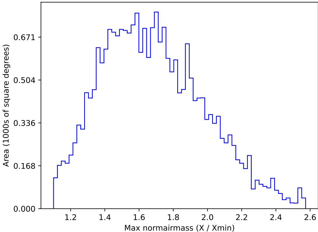
weather_cloudso10v3.4_10yrs All sky u band: Max normairmass
