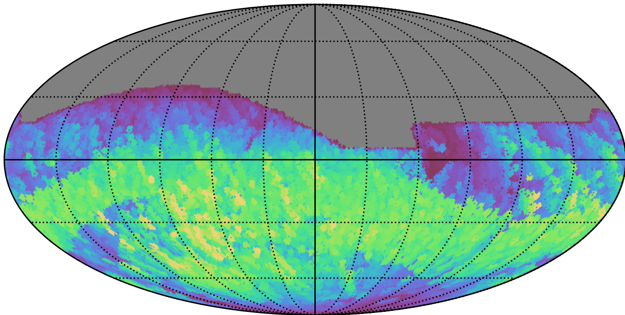
weather_cloudso10v3.4_10yrs All sky r band: Max normairmass
