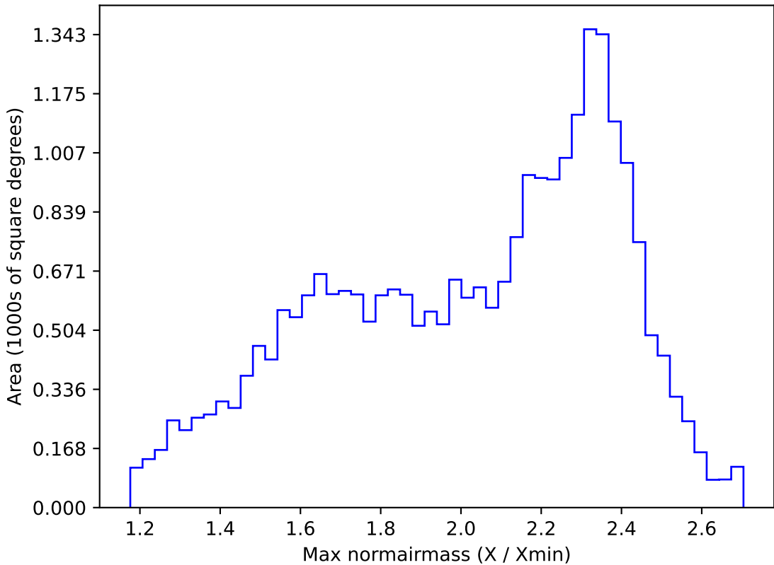
weather_cloudso10v3.4_10yrs All sky r band: Max normairmass
