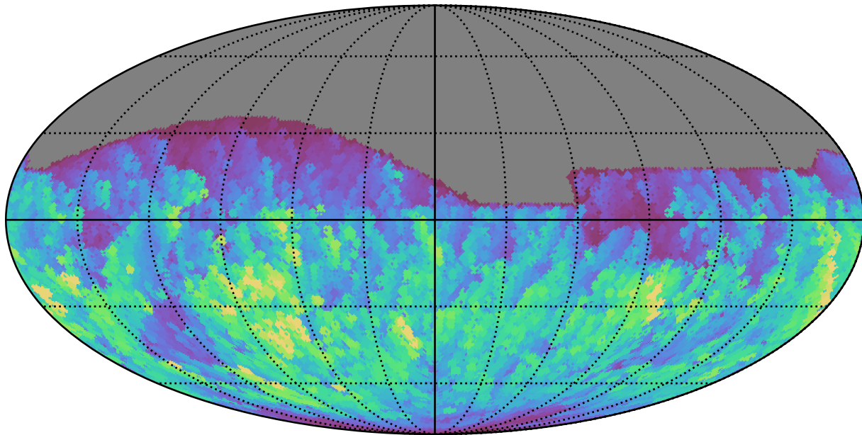
weather_cloudso10v3.4_10yrs All sky g band: Max normairmass
