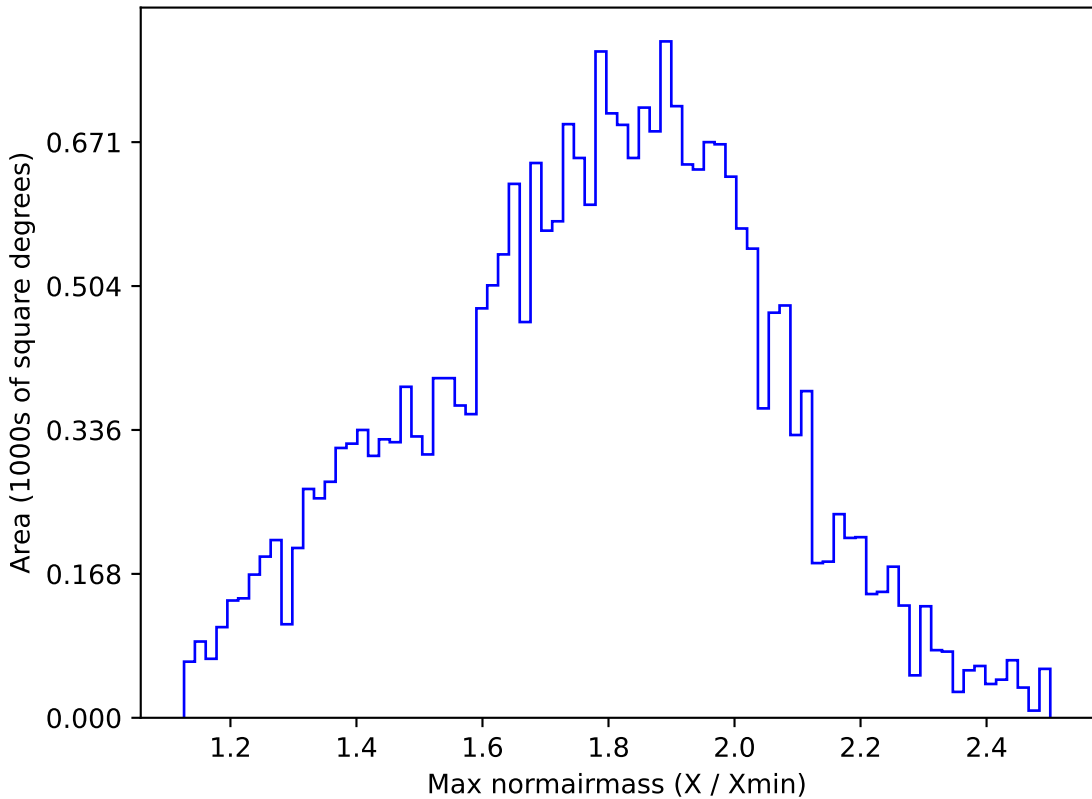
weather_cloudso10v3.4_10yrs All sky g band: Max normairmass
