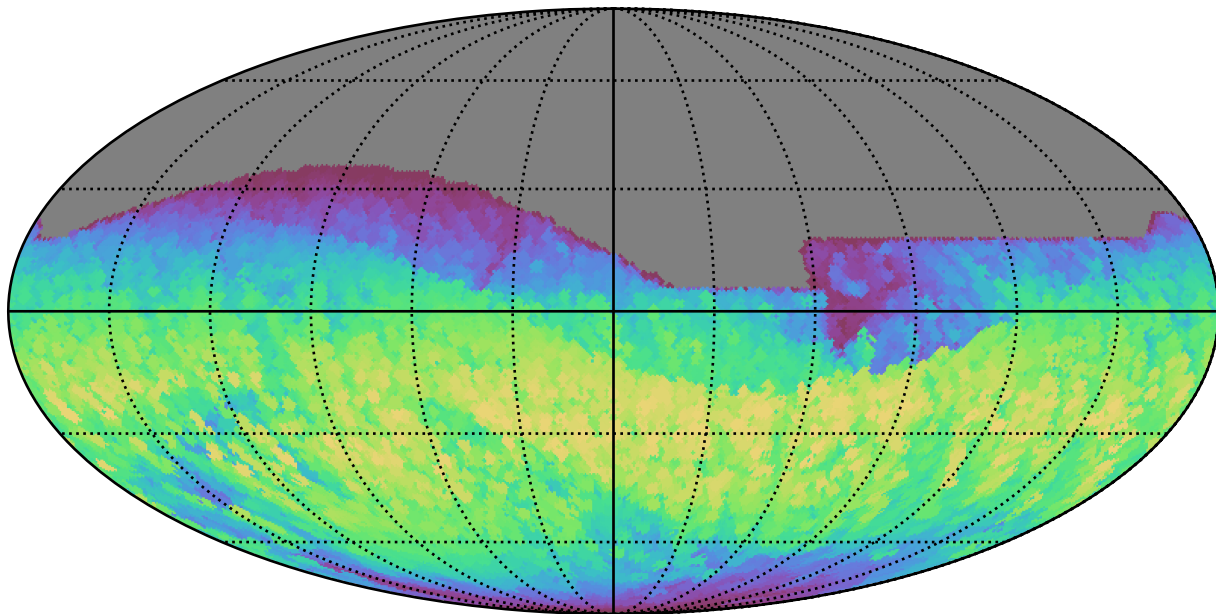
weather_cloudso10v3.4_10yrs All sky all bands: Max normairmass
