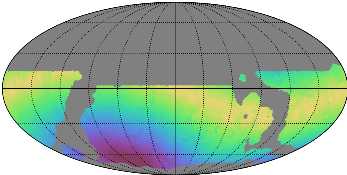
weather_cloudso10v3.4_10yrs WFD z band: Max moonDistance
