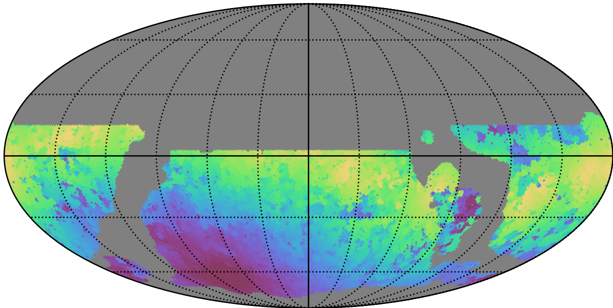
weather_cloudso10v3.4_10yrs WFD y band: Max moonDistance
