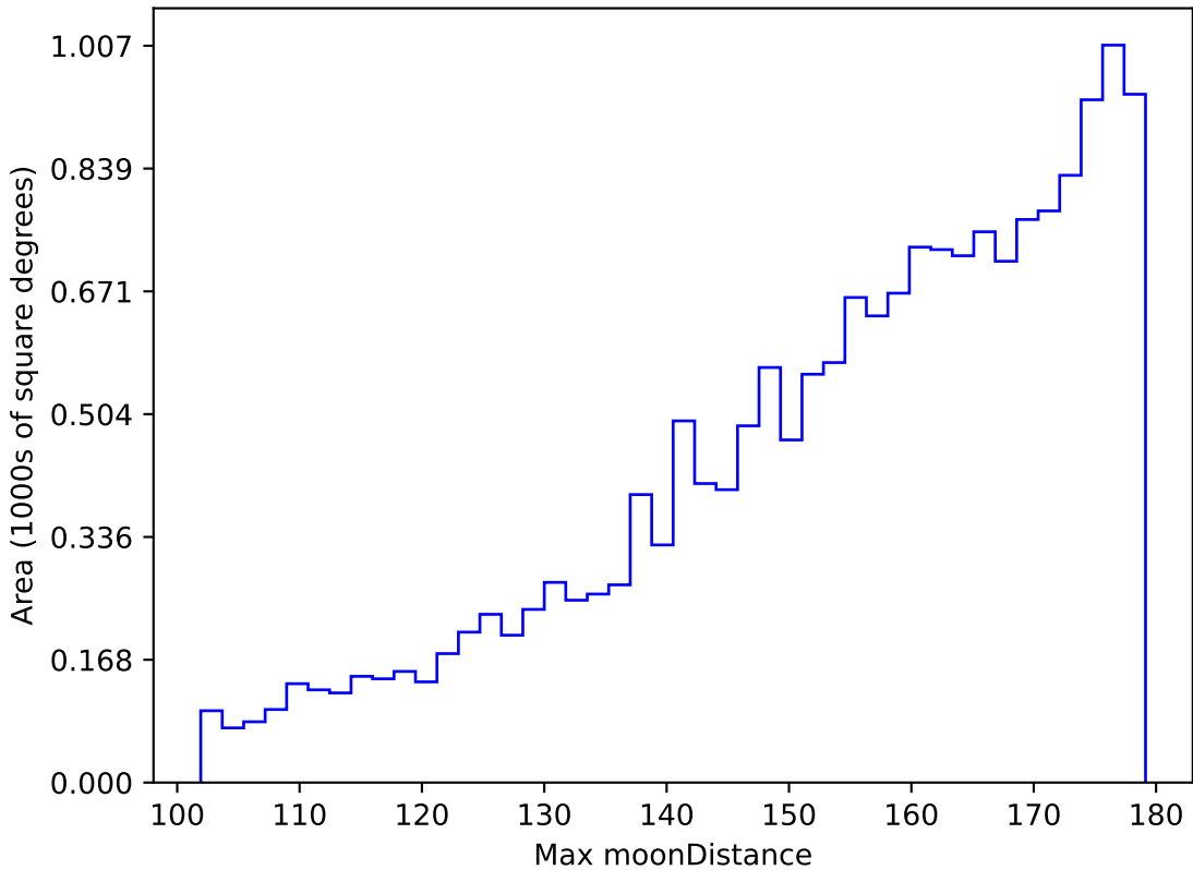
weather_cloudso10v3.4_10yrs WFD u band: Max moonDistance
