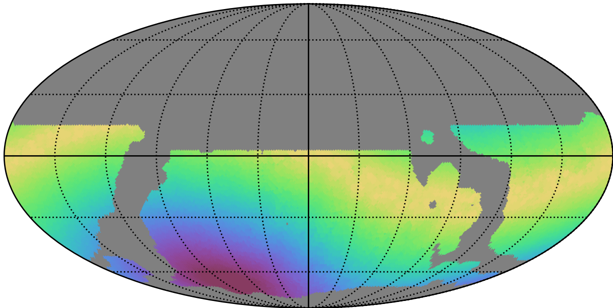
weather_cloudso10v3.4_10yrs WFD r band: Max moonDistance
