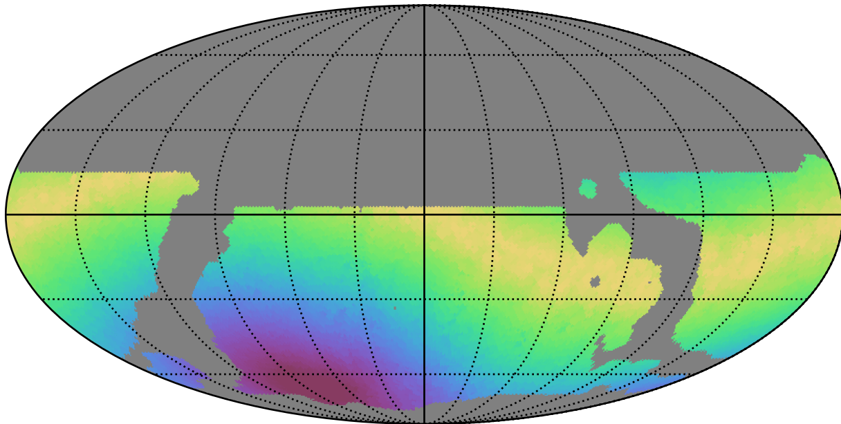
weather_cloudso10v3.4_10yrs WFD i band: Max moonDistance
