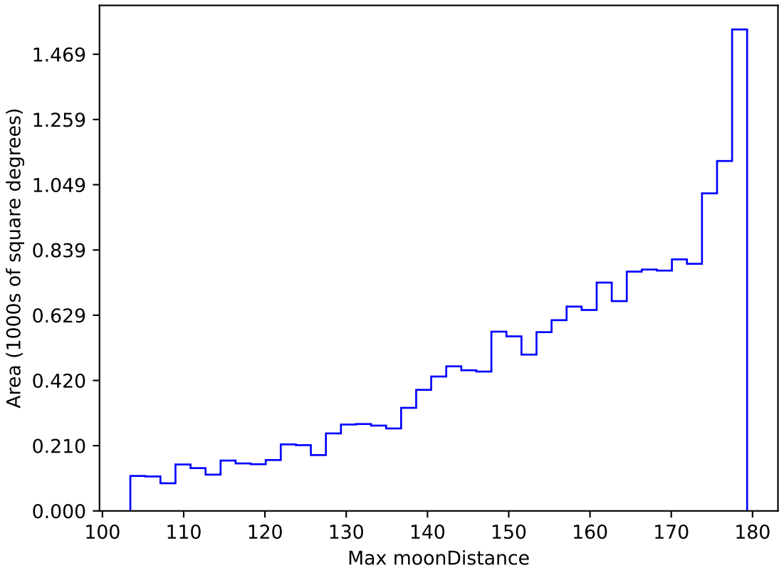
weather_cloudso10v3.4_10yrs WFD i band: Max moonDistance
