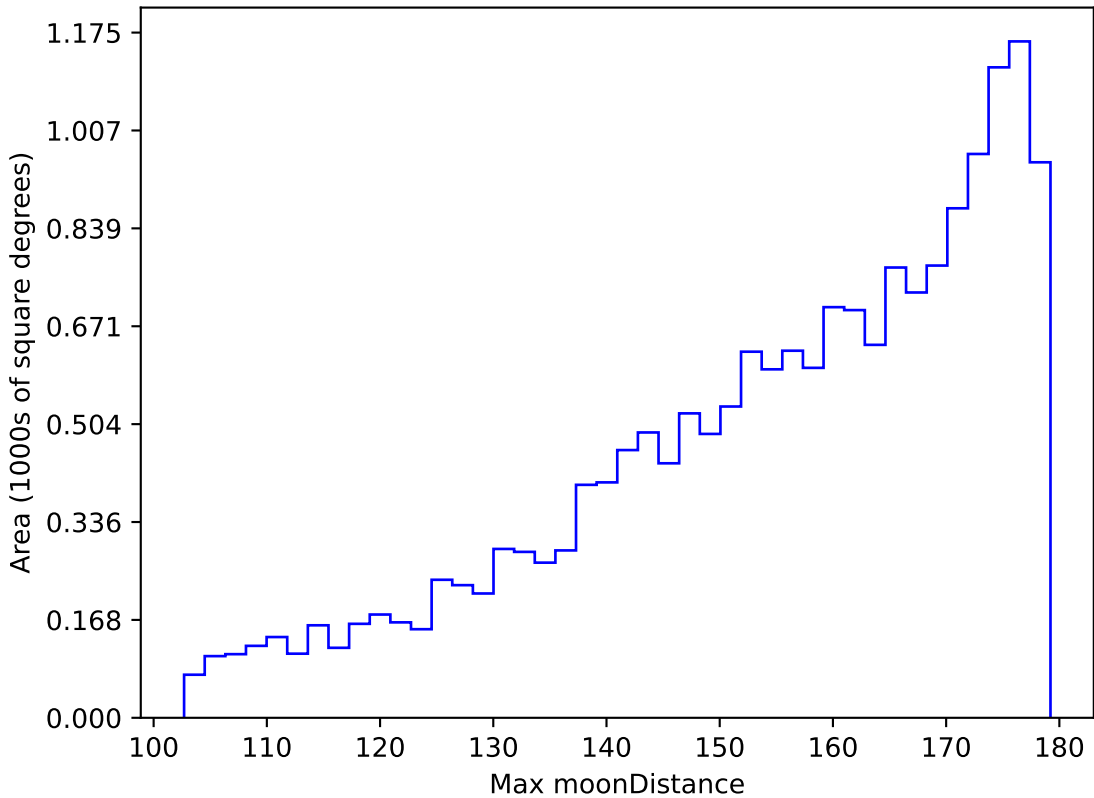
weather_cloudso10v3.4_10yrs WFD g band: Max moonDistance
