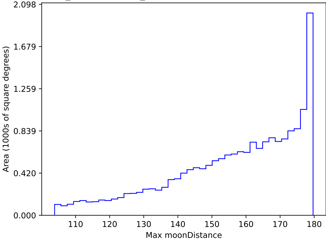
weather_cloudso10v3.4_10yrs WFD all bands: Max moonDistance
