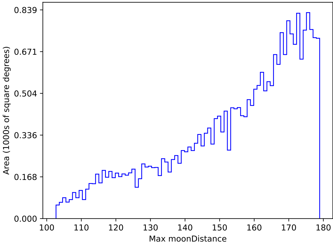
weather_cloudso10v3.4_10yrs All sky z band: Max moonDistance
