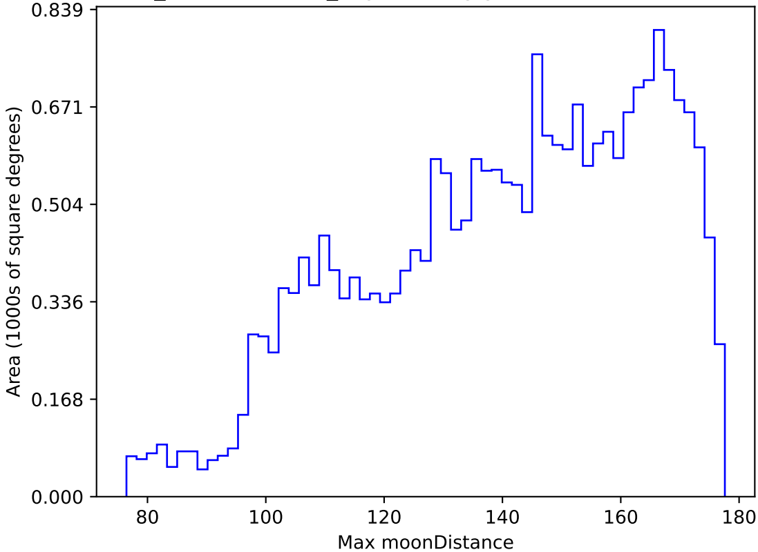
weather_cloudso10v3.4_10yrs All sky y band: Max moonDistance
