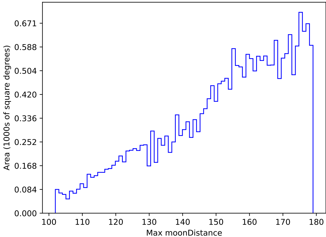
weather_cloudso10v3.4_10yrs All sky u band: Max moonDistance
