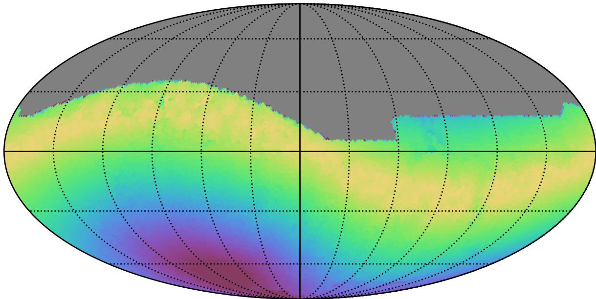
weather_cloudso10v3.4_10yrs All sky r band: Max moonDistance
