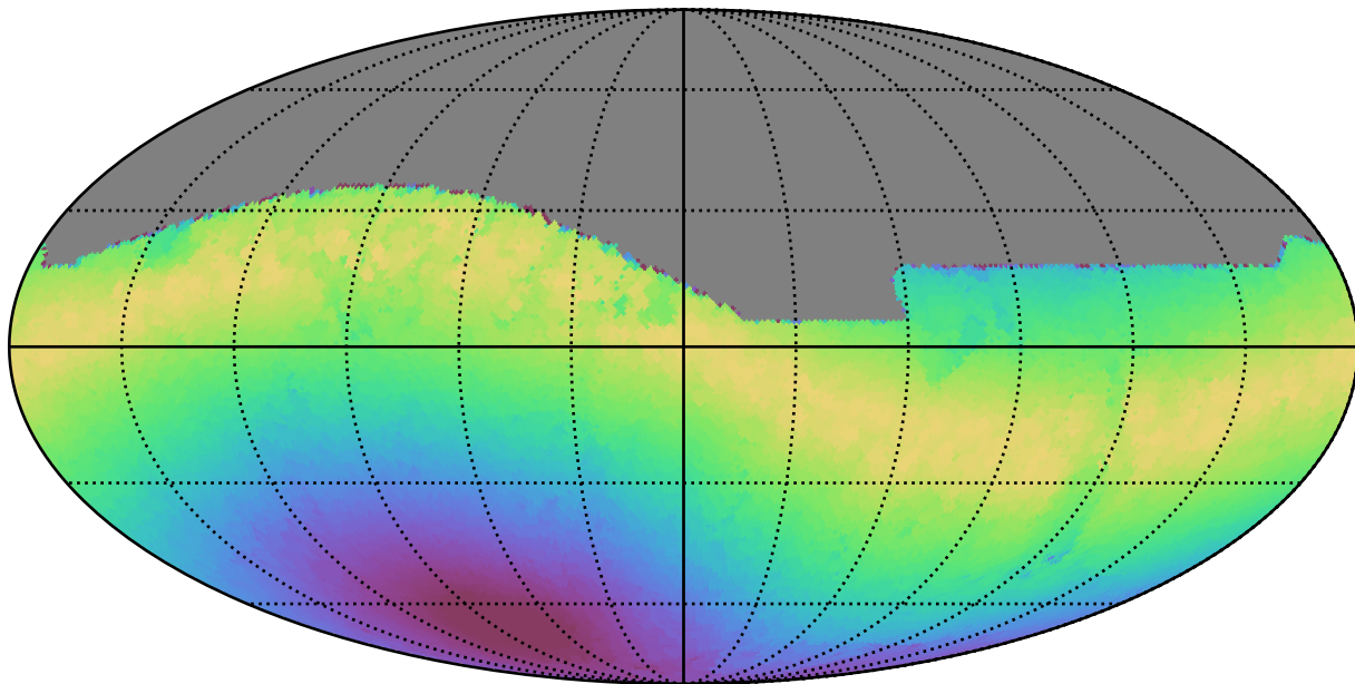
weather_cloudso10v3.4_10yrs All sky i band: Max moonDistance
