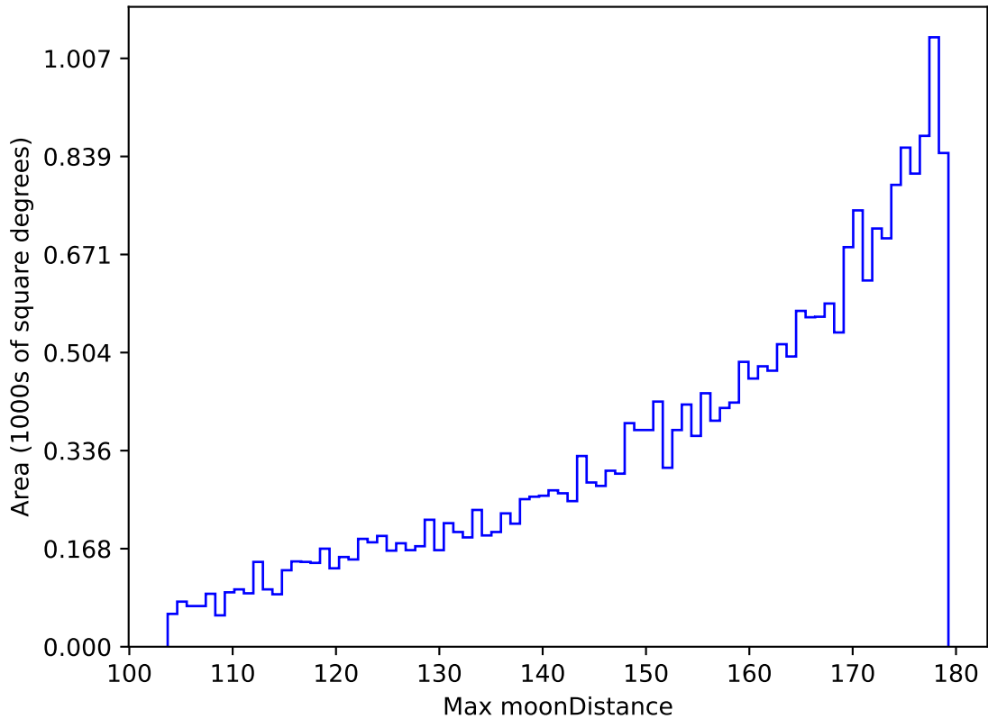
weather_cloudso10v3.4_10yrs All sky i band: Max moonDistance
