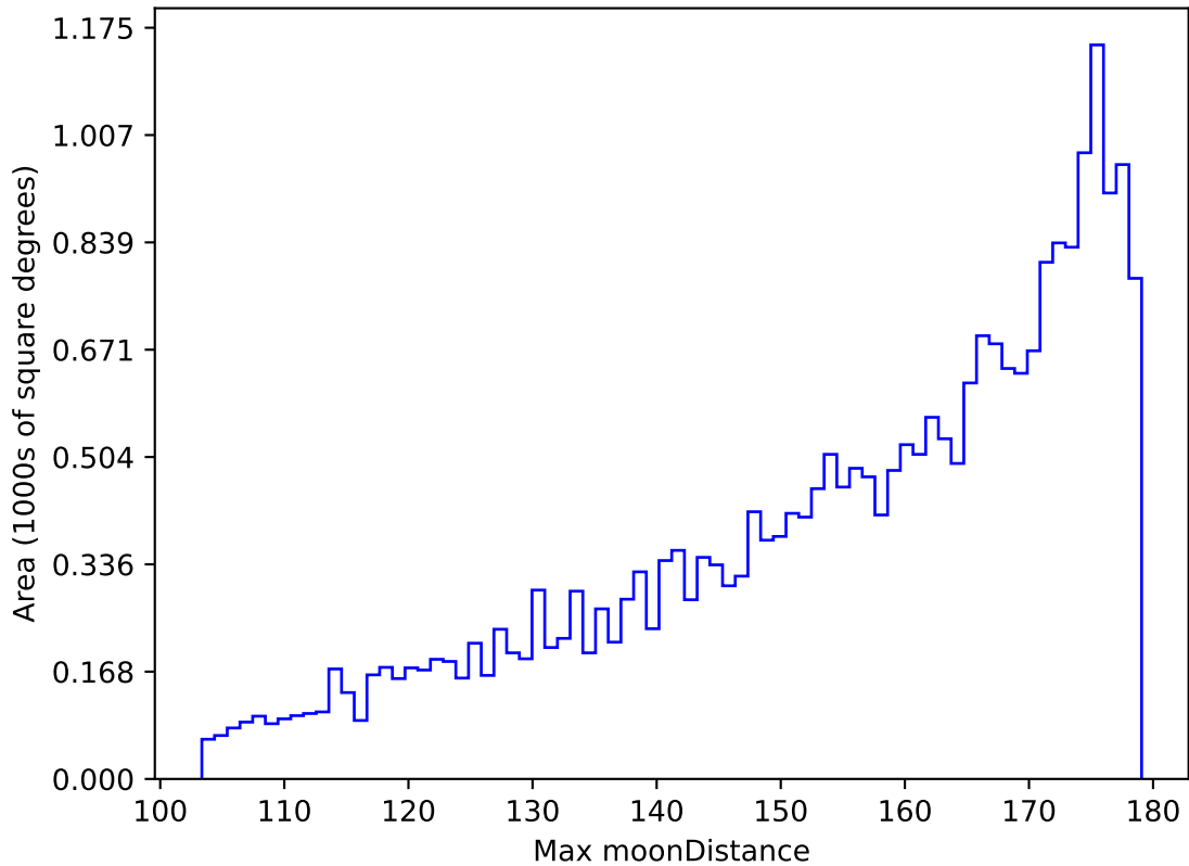
weather_cloudso10v3.4_10yrs All sky g band: Max moonDistance
