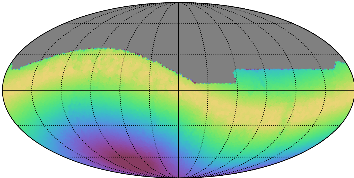
weather_cloudso10v3.4_10yrs All sky all bands: Max moonDistance
