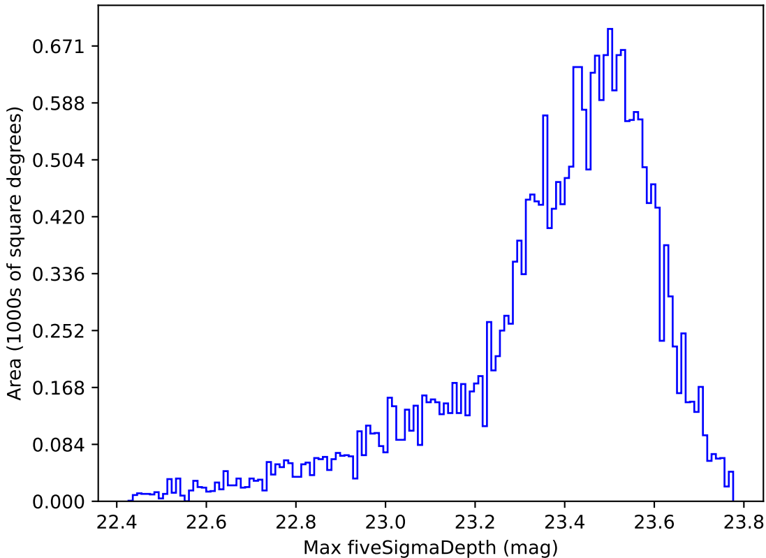
weather_cloudso10v3.4_10yrs Yr 1 z band: Max fiveSigmaDepth
