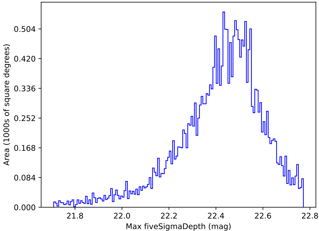
weather_cloudso10v3.4_10yrs Yr 1 y band: Max fiveSigmaDepth
