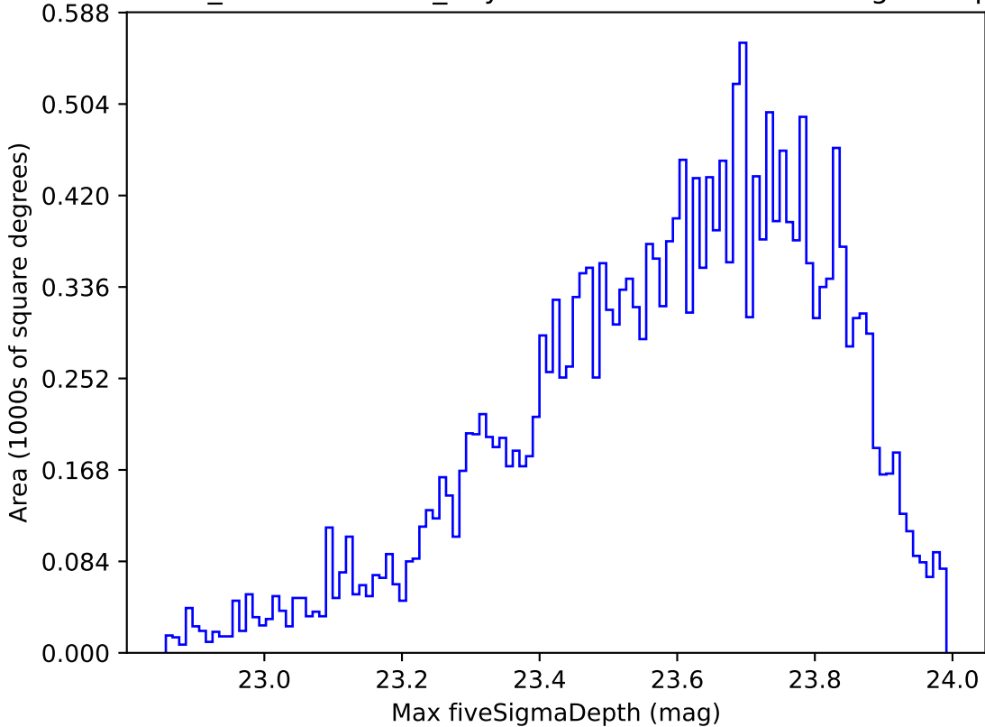
weather_cloudso10v3.4_10yrs Yr 1 u band: Max fiveSigmaDepth
