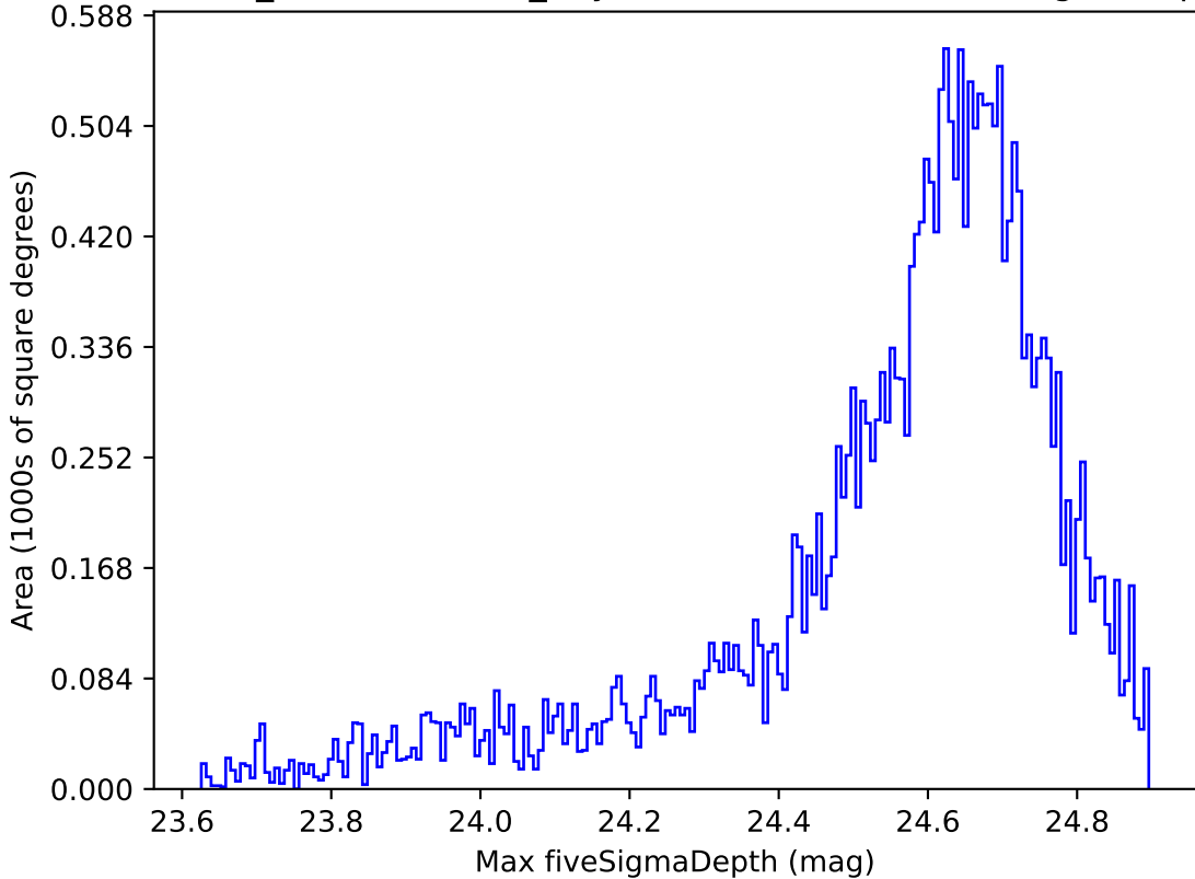
weather_cloudso10v3.4_10yrs Yr 1 r band: Max fiveSigmaDepth
