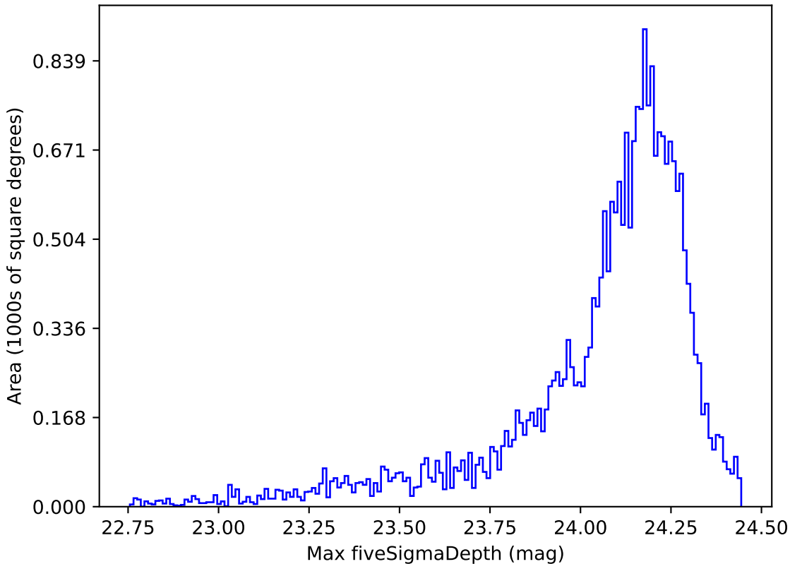
weather_cloudso10v3.4_10yrs Yr 1 i band: Max fiveSigmaDepth
