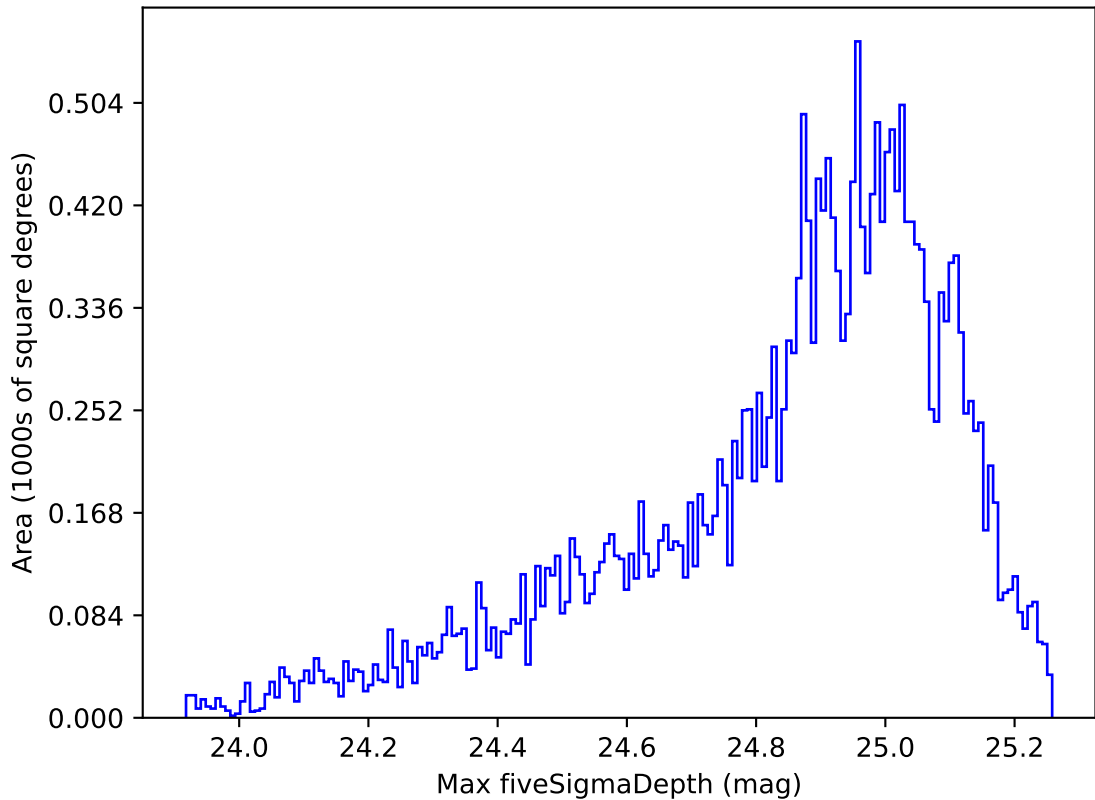
weather_cloudso10v3.4_10yrs Yr 1 g band: Max fiveSigmaDepth
